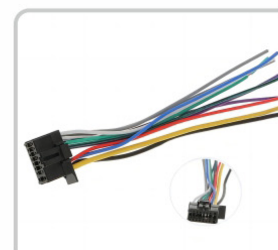
16 PIN BLACK PLUG AUTO RADIO LINE CONNECTOR REPLACEMENT WIRING HARNESS
